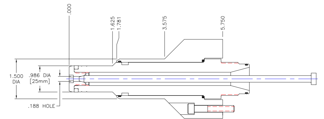
MODEL #SN714-10A DIVING NOZZLE (25mm DIA.) WITH SCREW IN TIP
