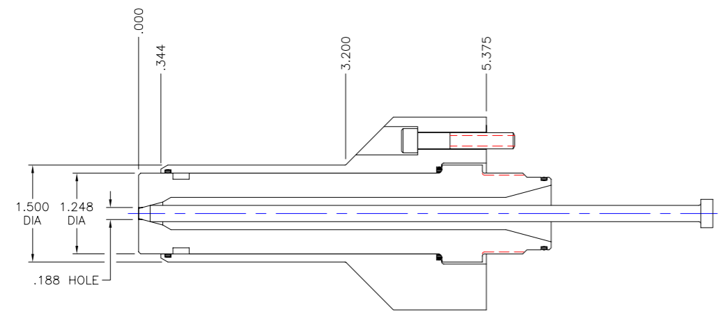
MODEL #SN714-3A FLAT-TIP NOZZLE STANDARD LENGTH
