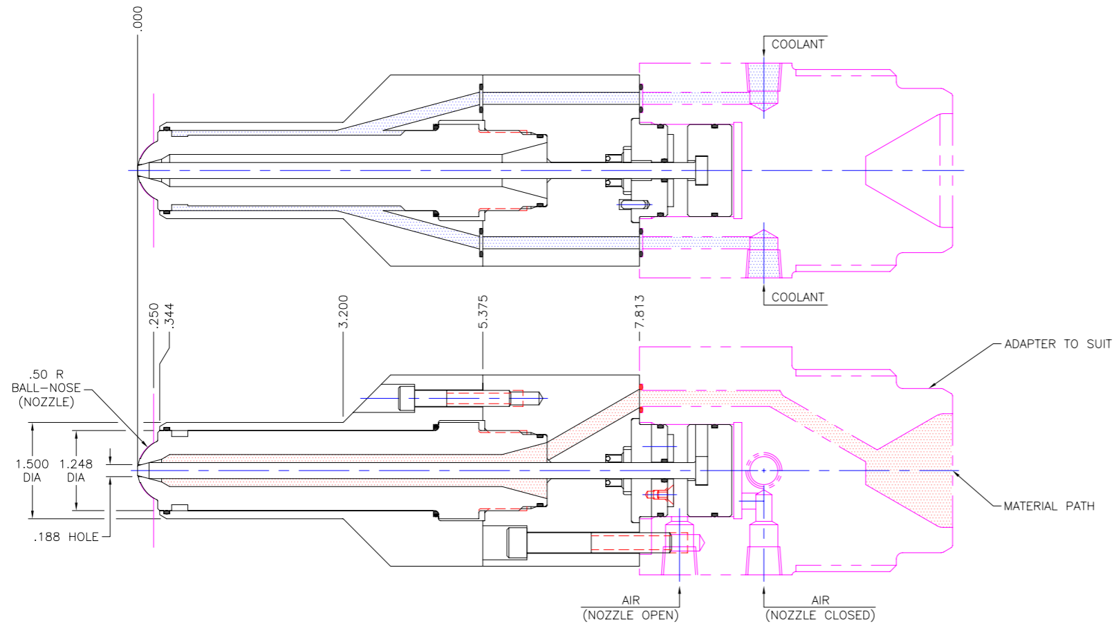
MODEL #SN714-1A 1/2" BALL NOSE NOZZLE (.750 DIA) STANDARD LENGTH
